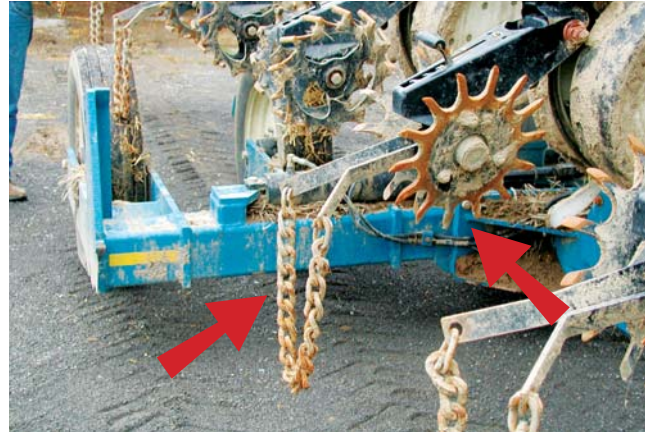
Spading/closing wheels with optional drag chain.
