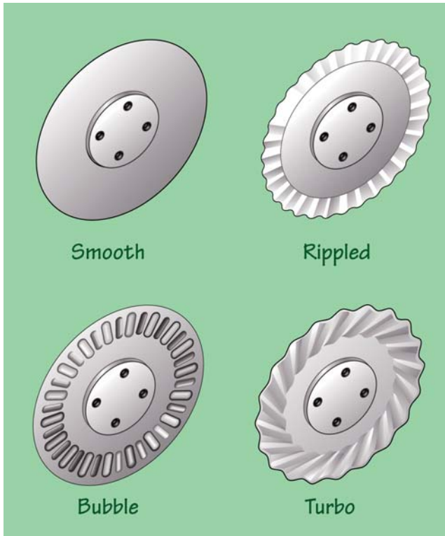
Smooth, rippled, bubble, and fluted turbo-coulters.
