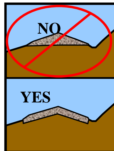
Figure 2. Road base preparation.
